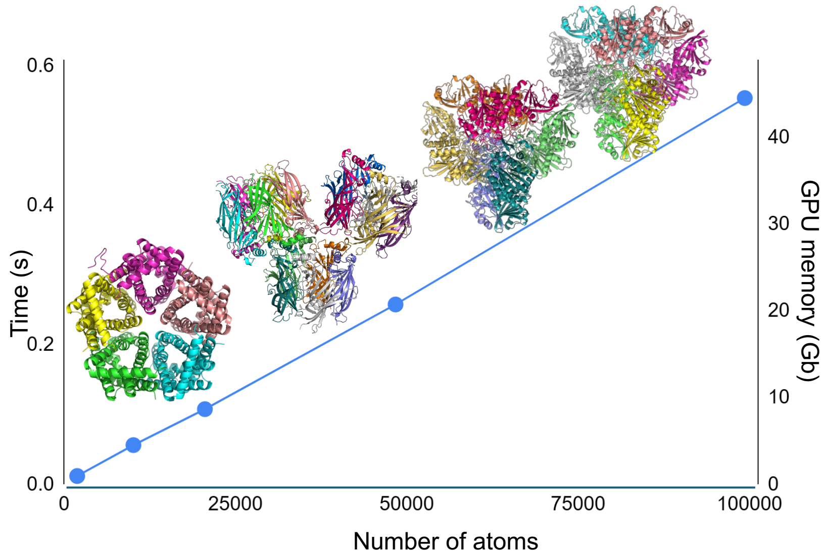
Figure 2. Computational scaling of the AIMNet2-QR model.
