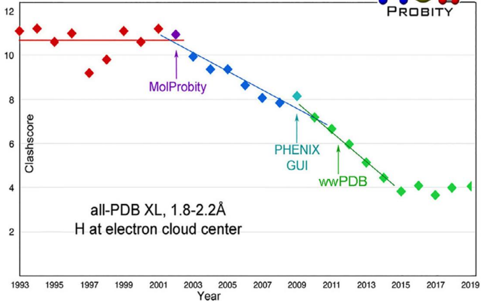
ALL-atom Clashscore vs Year
